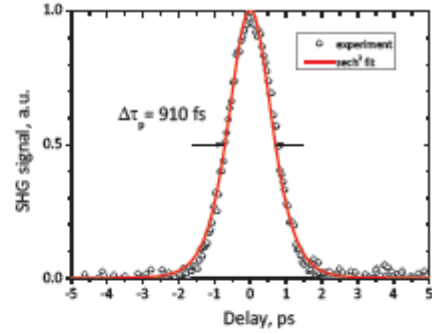
Autocorrelation trace at maximum power
