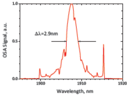
Normalized spectrum at maximum power
